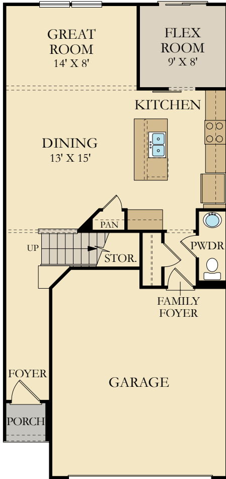
FIRST FLOOR
